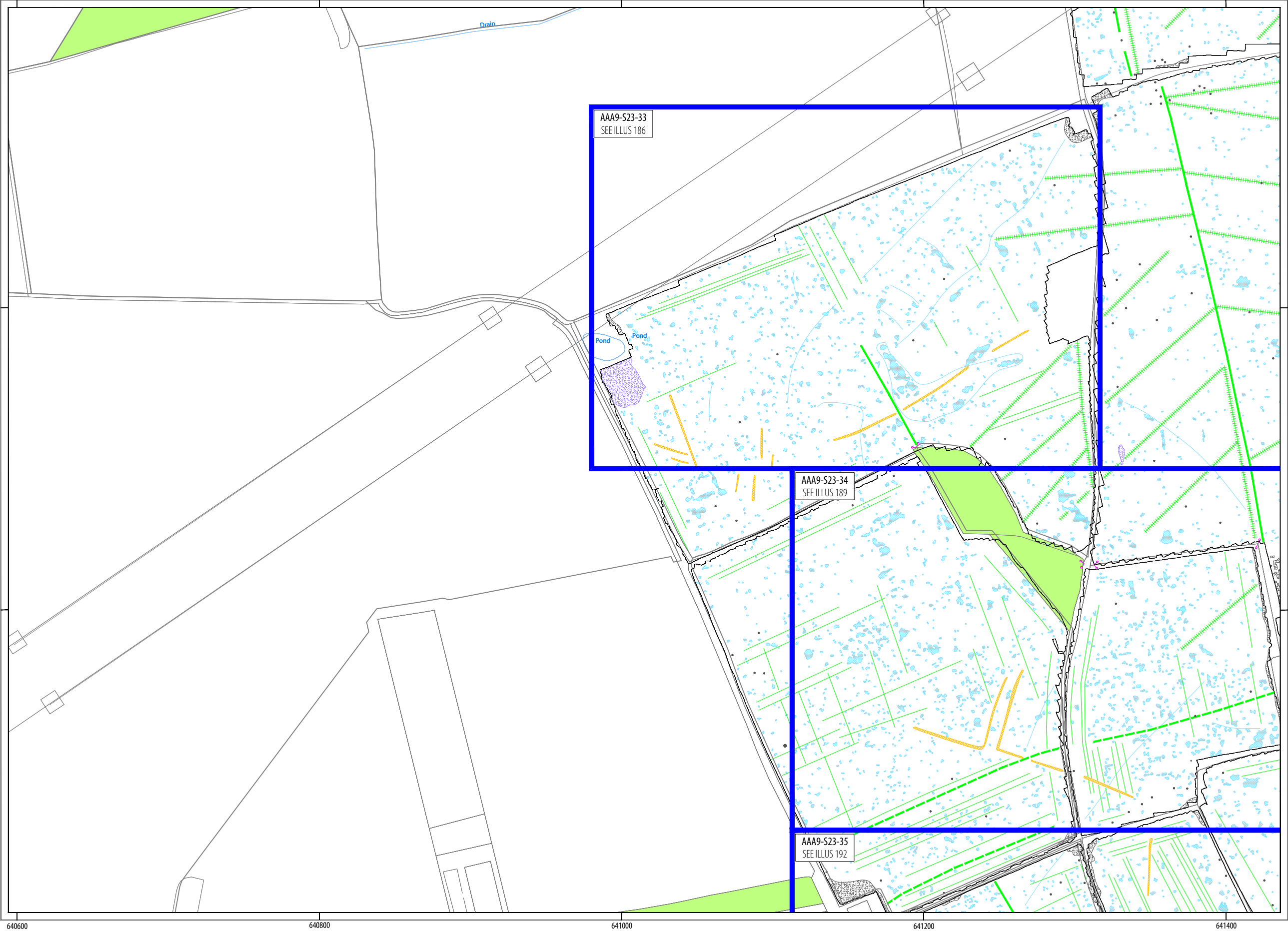
ILLUS 78 Interpretation of magnetometer data; Sector 23
