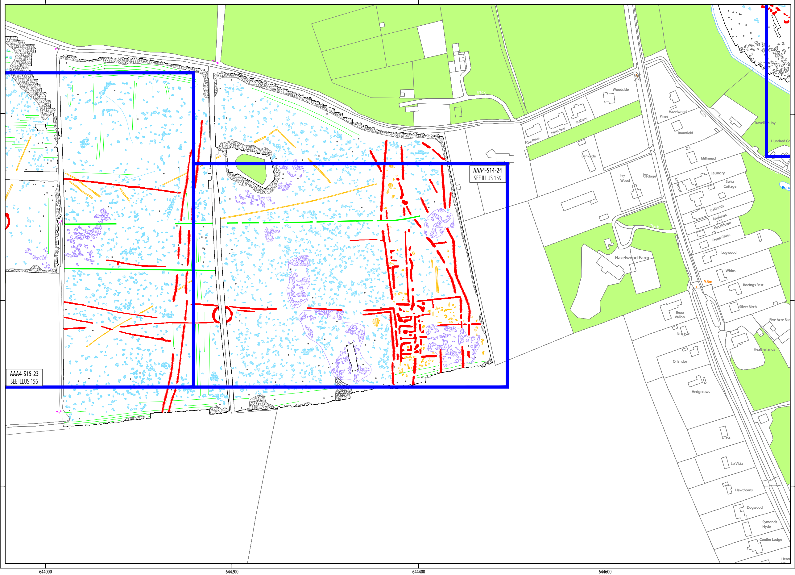
ILLUS 51 Interpretation of magnetometer data; Sector 14
