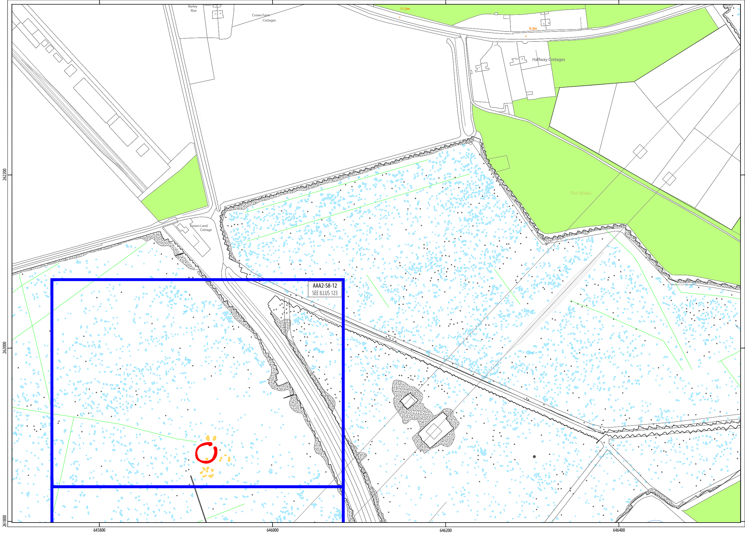
ILLUS 33 Interpretation of magnetometer data; Sector 8
