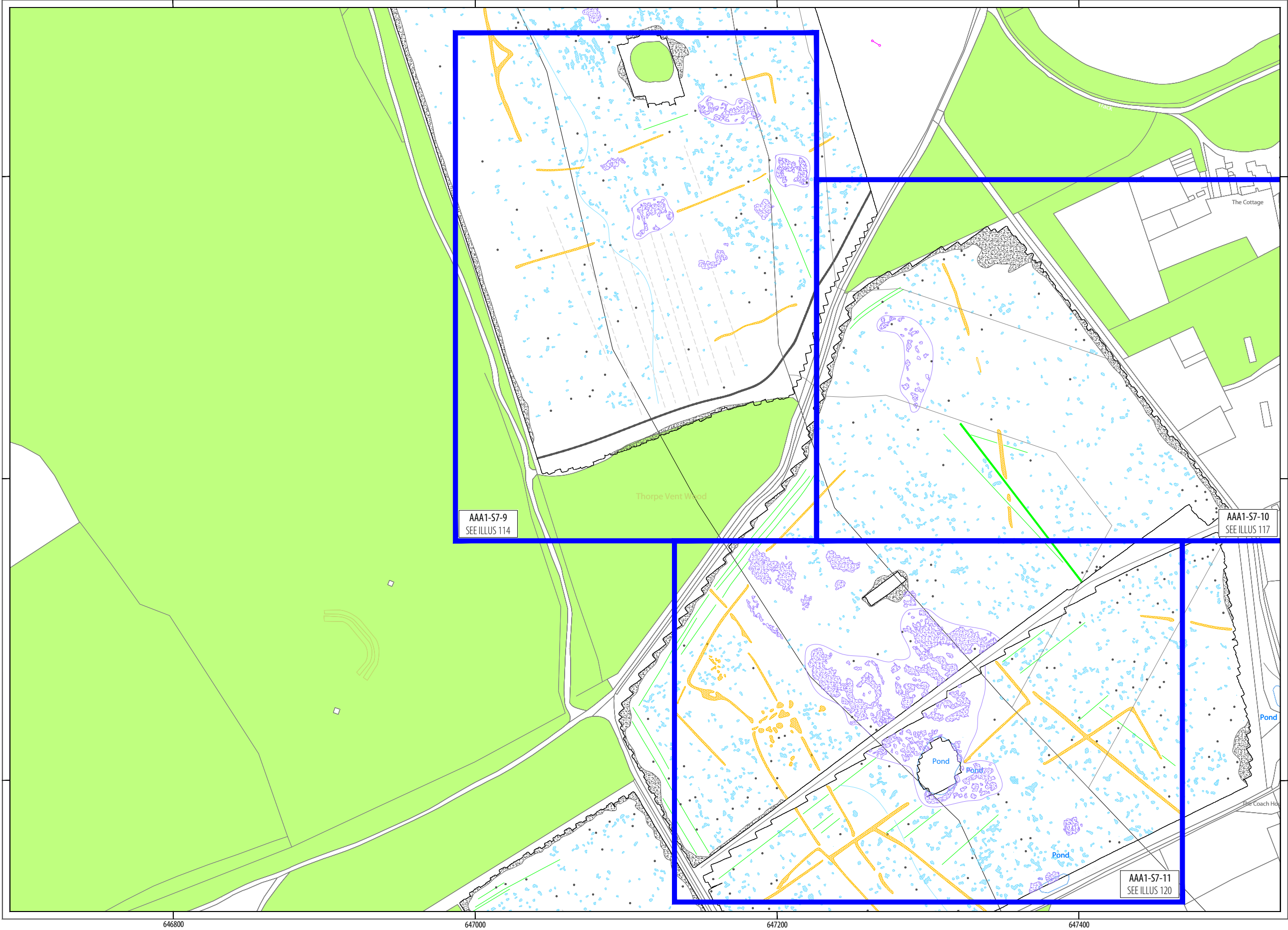
ILLUS 30 Interpretation of magnetometer data; Sector 7
