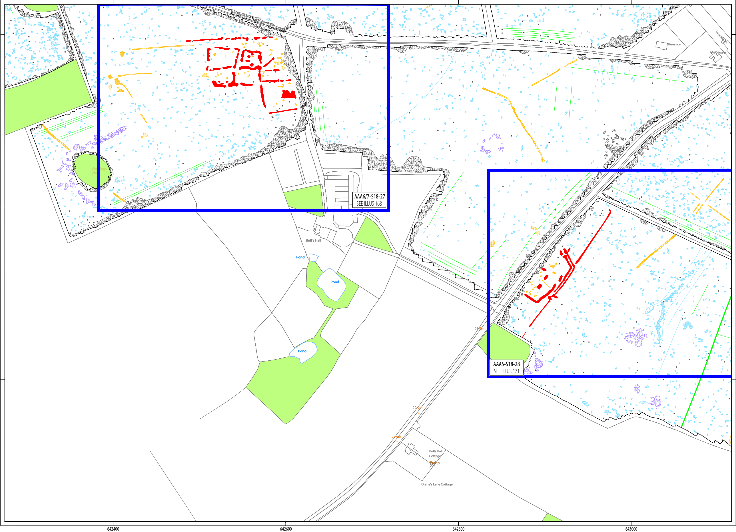
ILLUS 63 Interpretation of magnetometer data; Sector 18
