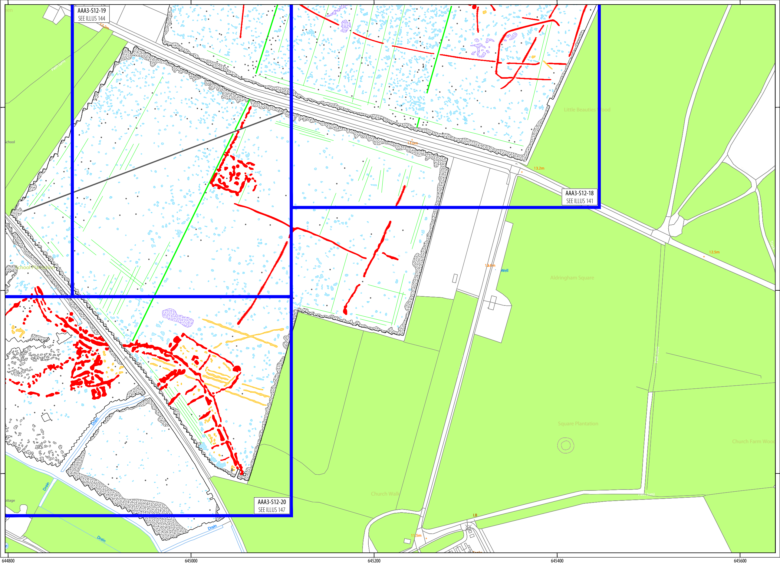
ILLUS 45 Interpretation of magnetometer data; Sector 12
