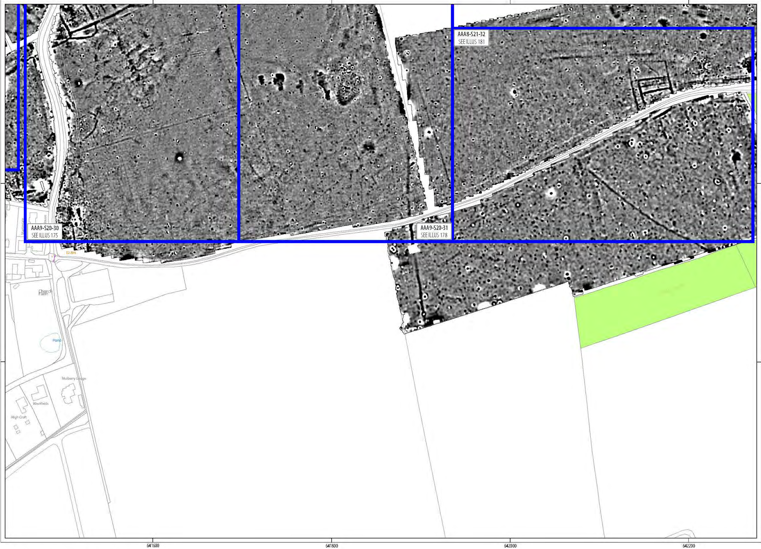
ILLUS 70 Processed greyscale magnetometer data; Sector 21
