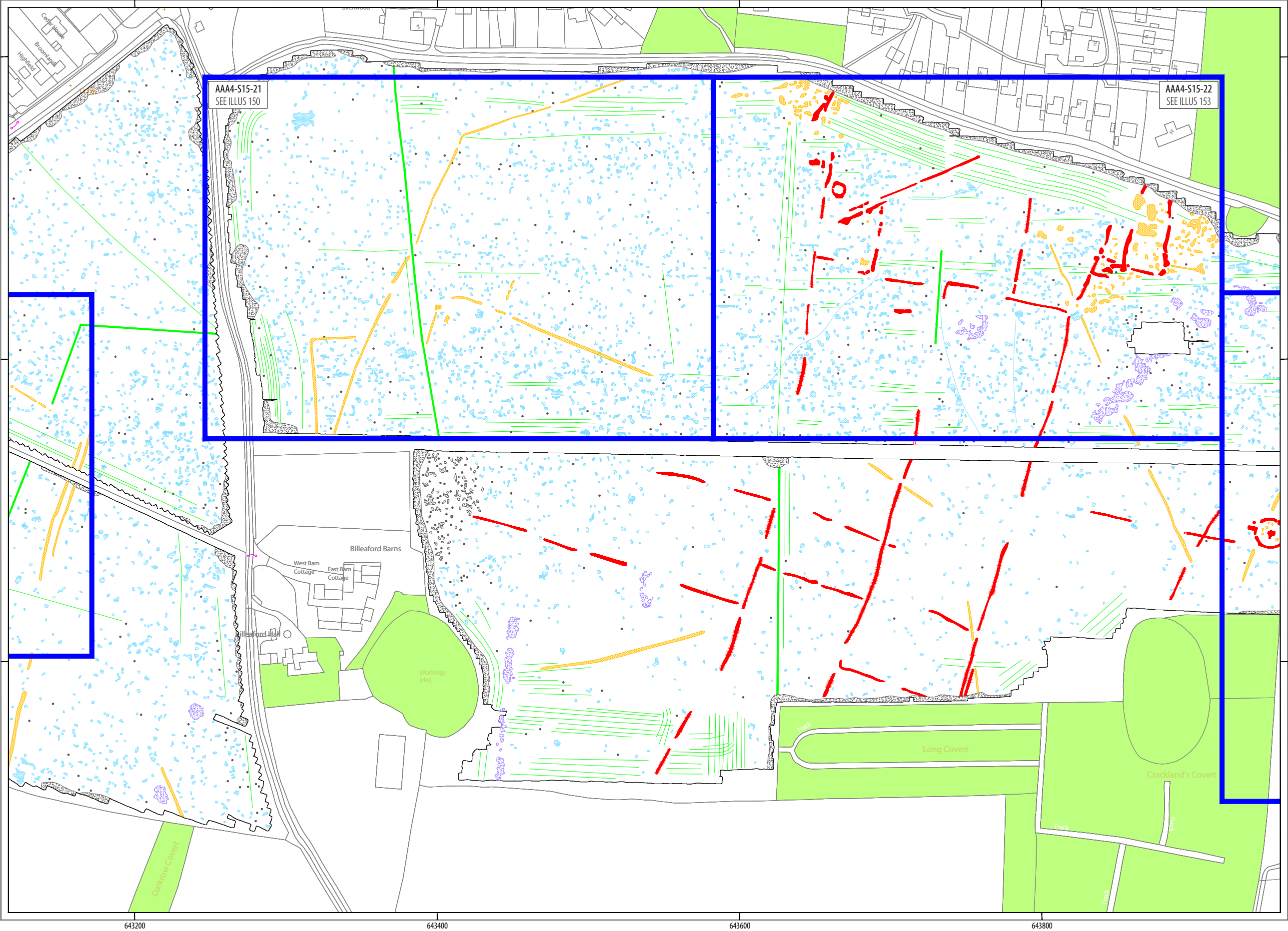
ILLUS 54 Interpretation of magnetometer data; Sector 15
